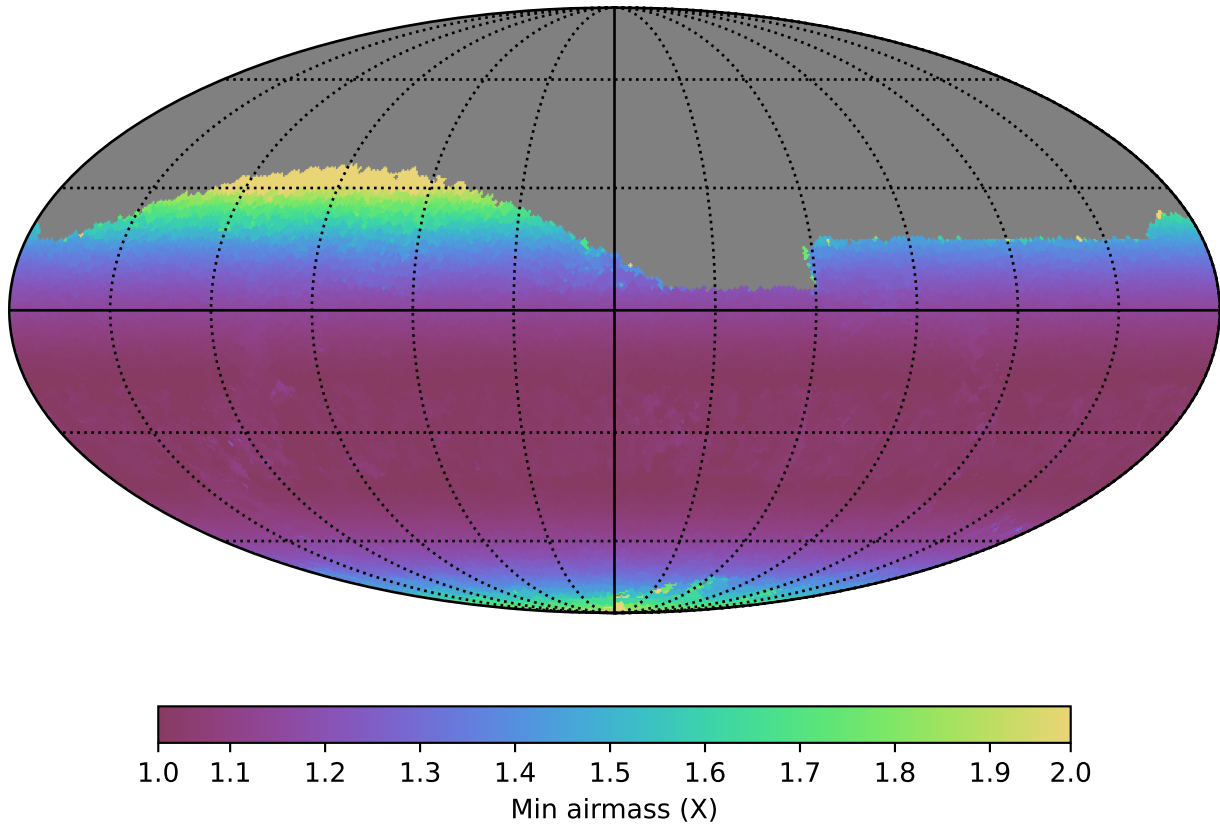
too_5_4v3.4_10yrs Yr 1 r band: Min airmass
