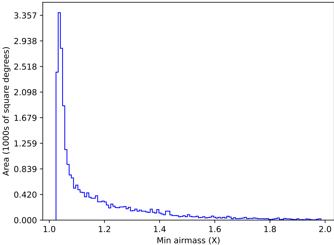
too_5_4v3.4_10yrs Yr 1 r band: Min airmass
