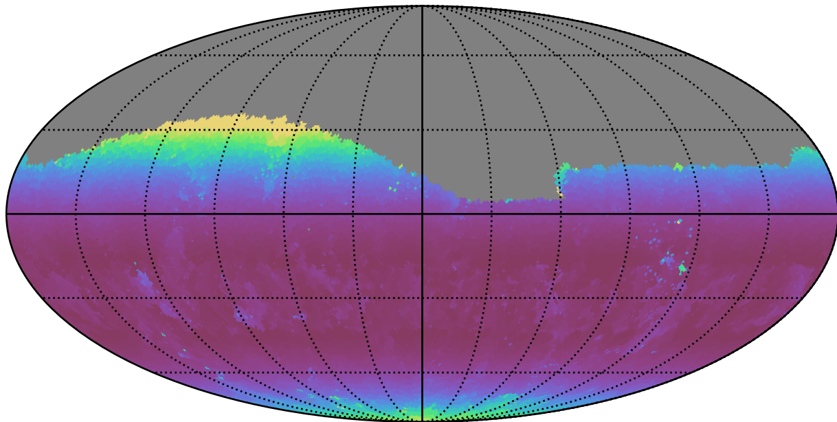
too_5_4v3.4_10yrs Yr 1 g band: Min airmass
