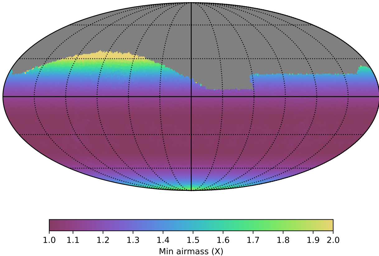
too_5_4v3.4_10yrs Yr 1 all bands: Min airmass
