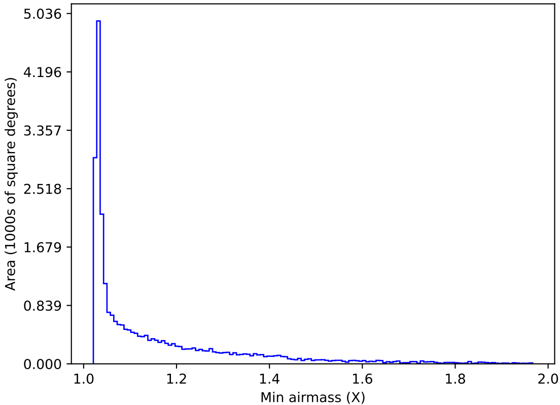
too_5_4v3.4_10yrs Yr 1 all bands: Min airmass
