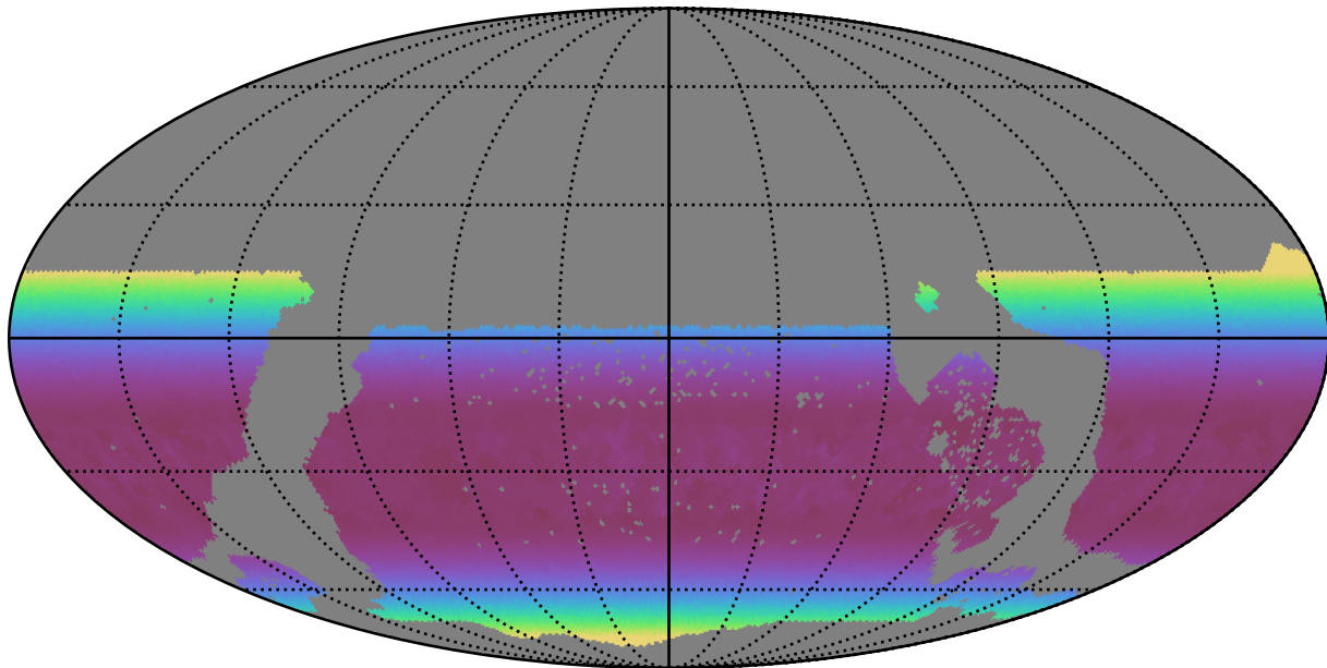
too_5_4v3.4_10yrs WFD z band: Min airmass
