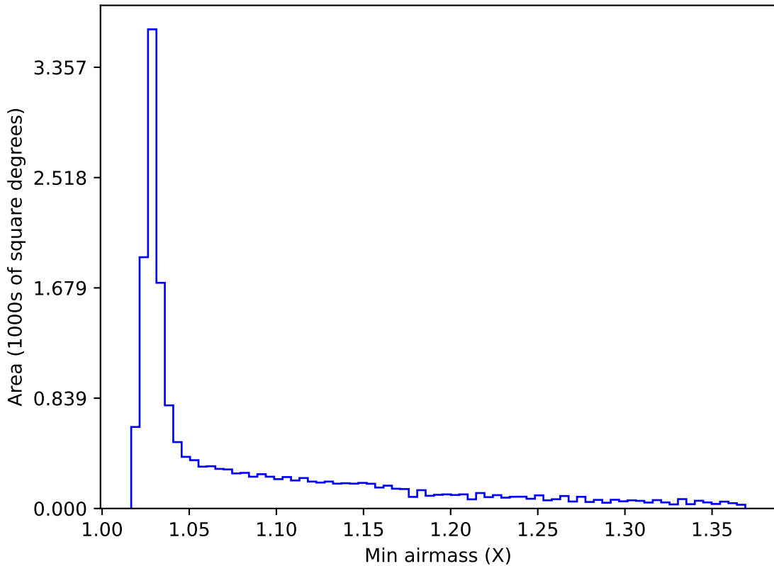
too_5_4v3.4_10yrs WFD z band: Min airmass
