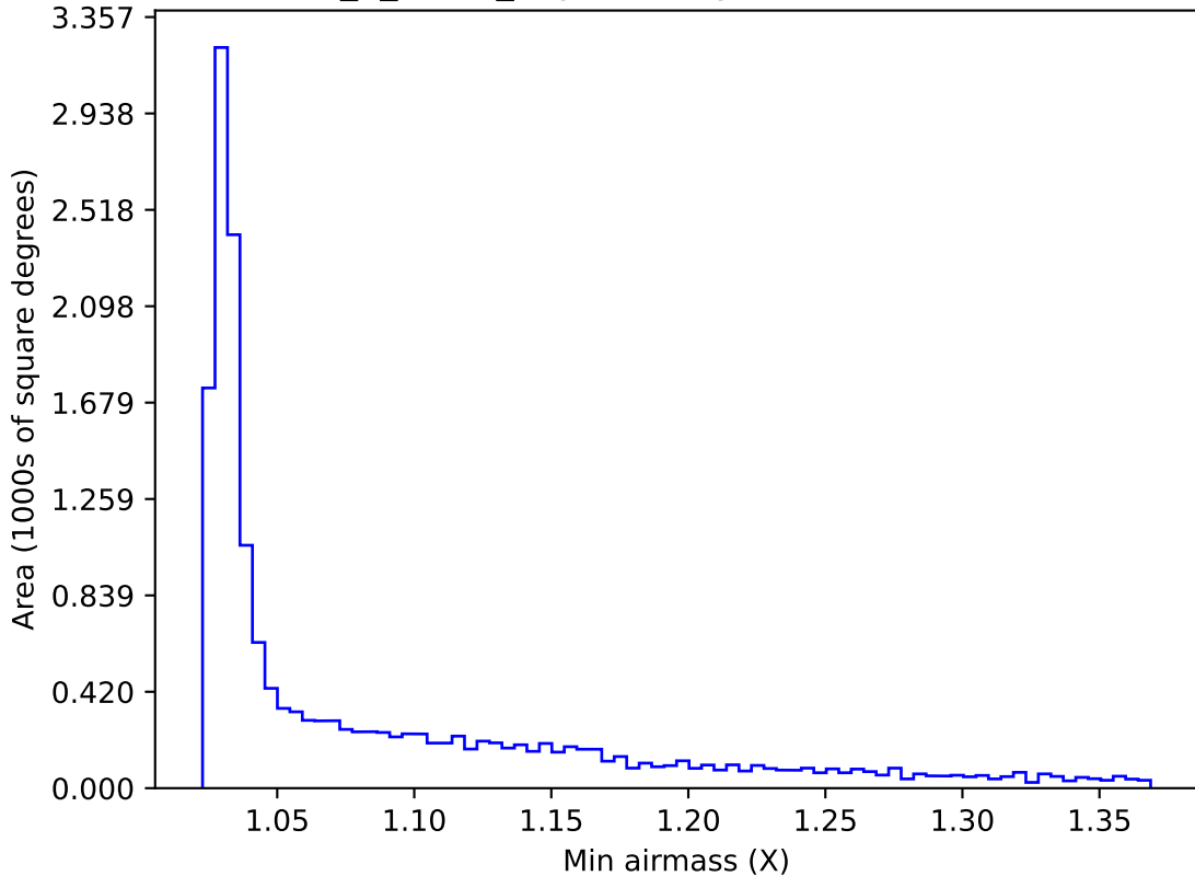
too_5_4v3.4_10yrs WFD y band: Min airmass
