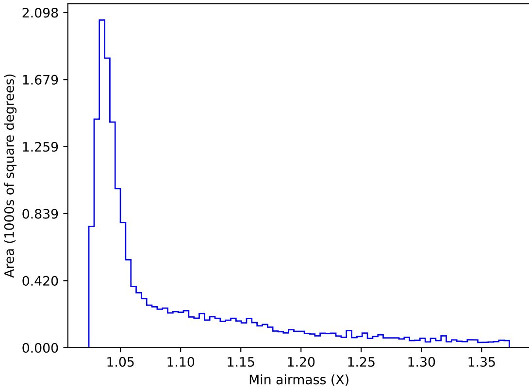
too_5_4v3.4_10yrs WFD u band: Min airmass
