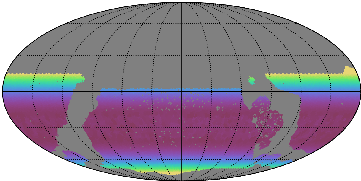
too_5_4v3.4_10yrs WFD r band: Min airmass
