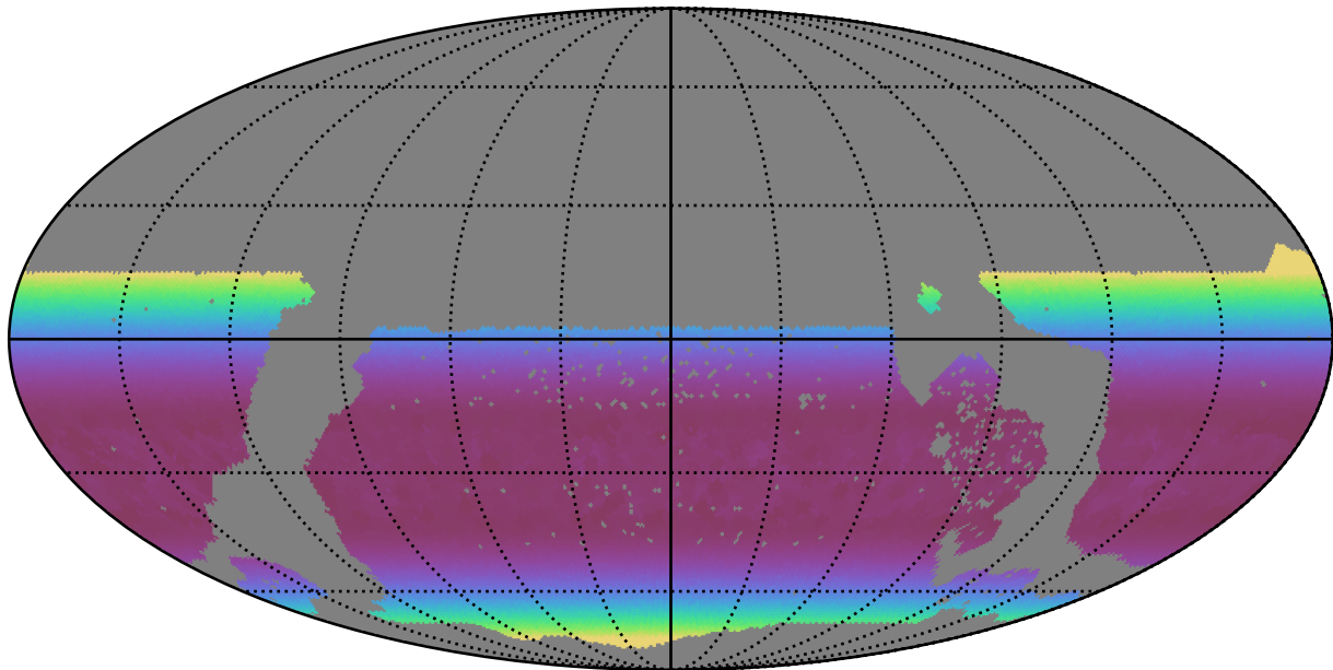
too_5_4v3.4_10yrs WFD i band: Min airmass
