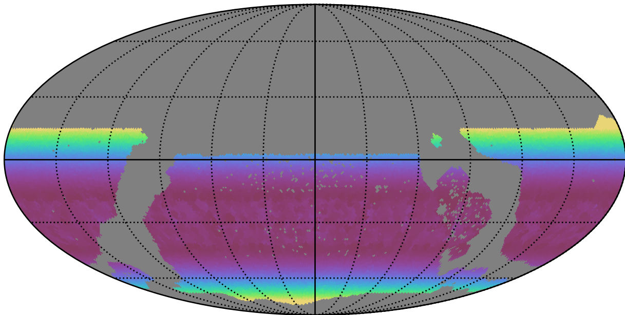
too_5_4v3.4_10yrs WFD g band: Min airmass
