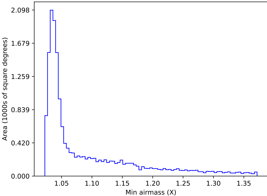
too_5_4v3.4_10yrs WFD g band: Min airmass
