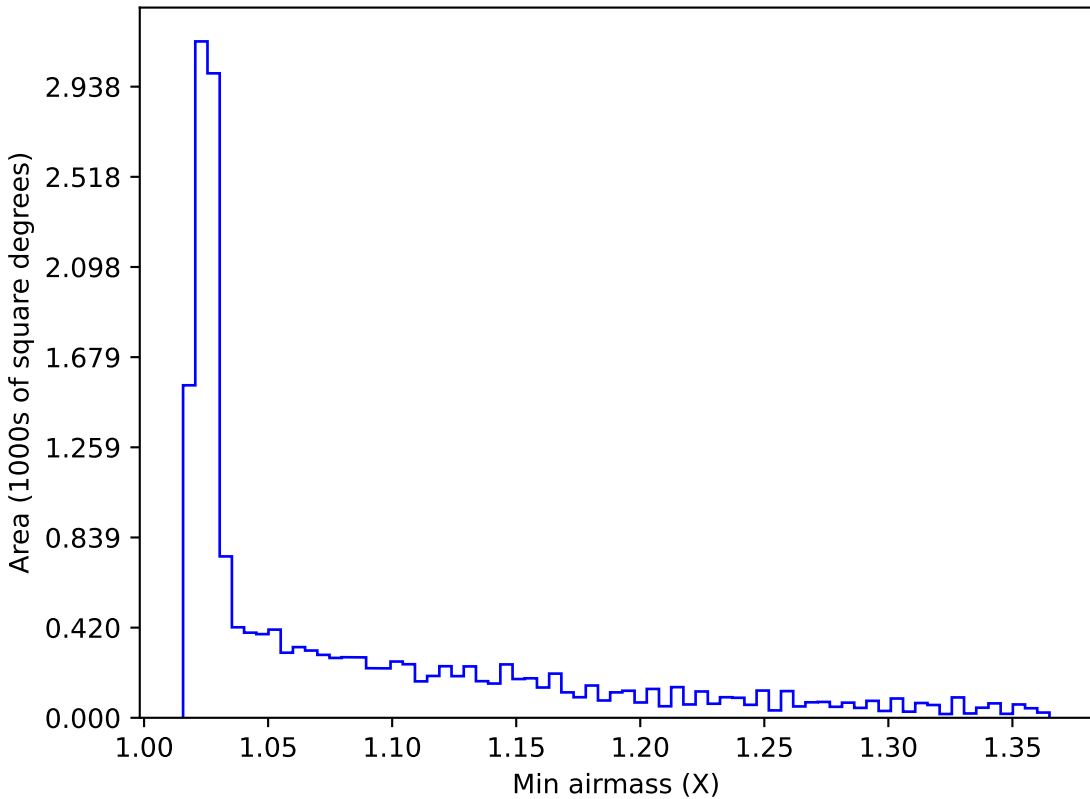
too_5_4v3.4_10yrs WFD all bands: Min airmass
