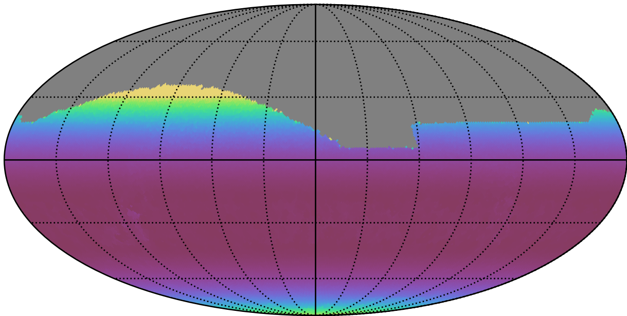
too_5_4v3.4_10yrs All sky z band: Min airmass
