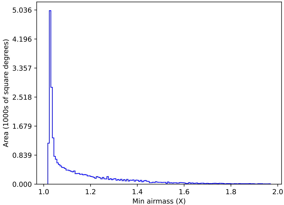
too_5_4v3.4_10yrs All sky z band: Min airmass
