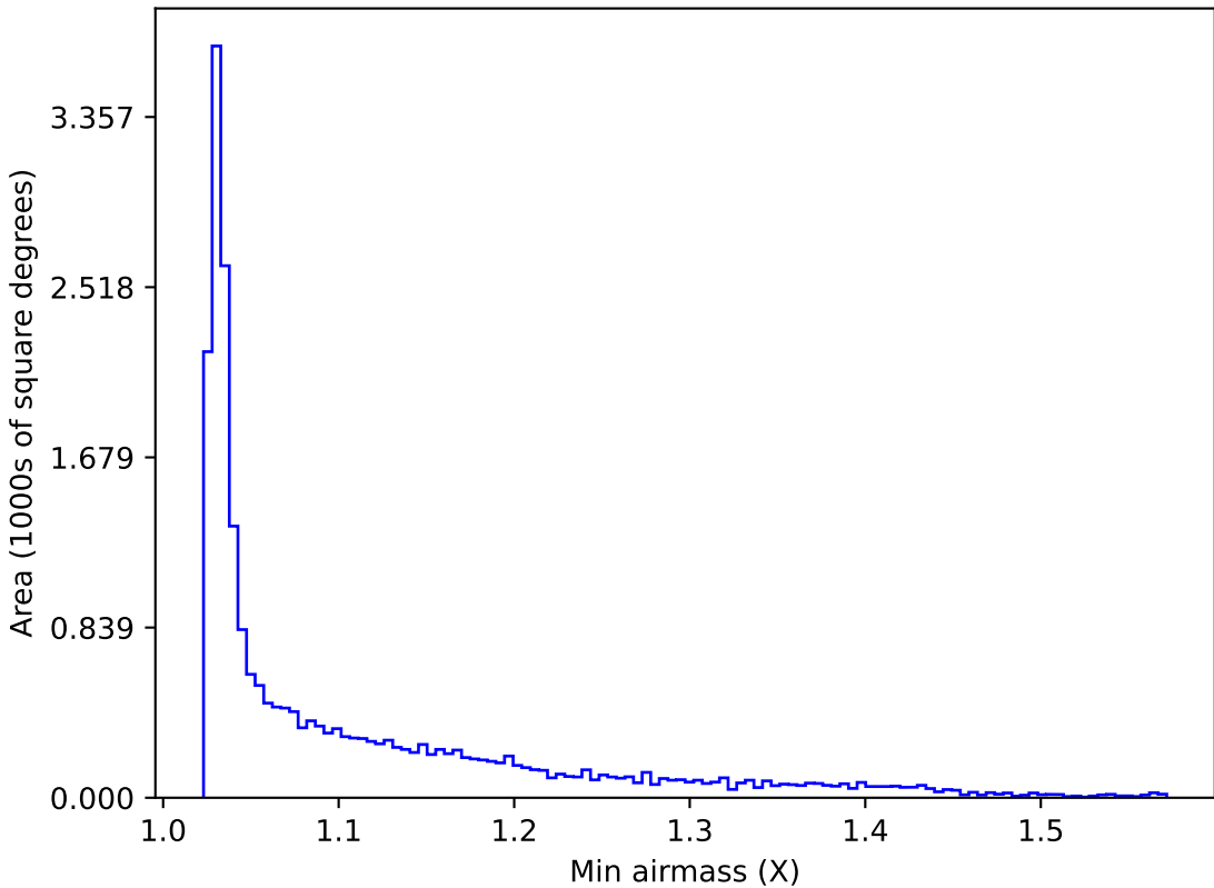
too_5_4v3.4_10yrs All sky y band: Min airmass
