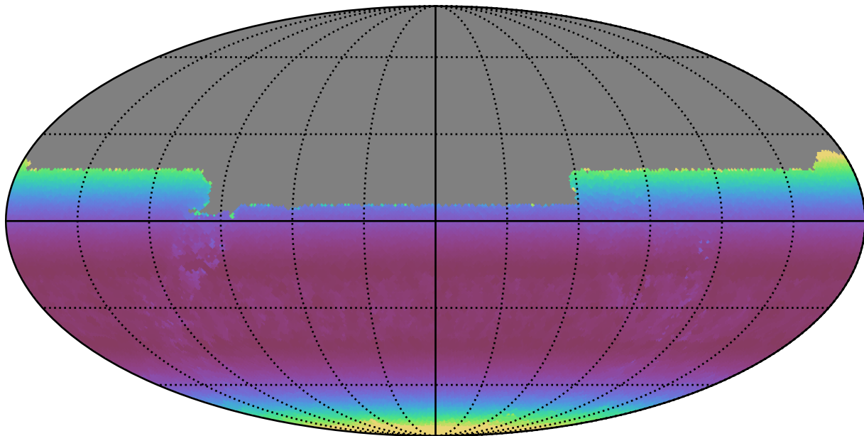
too_5_4v3.4_10yrs All sky u band: Min airmass
