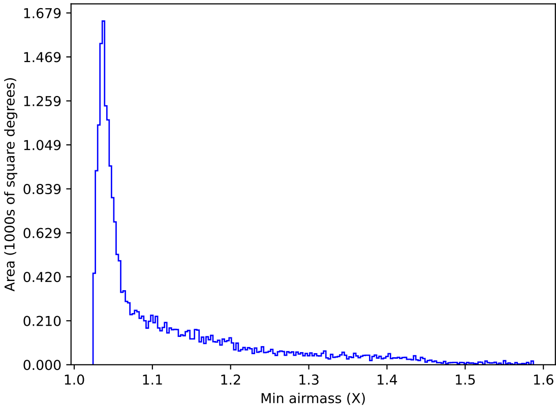
too_5_4v3.4_10yrs All sky u band: Min airmass
