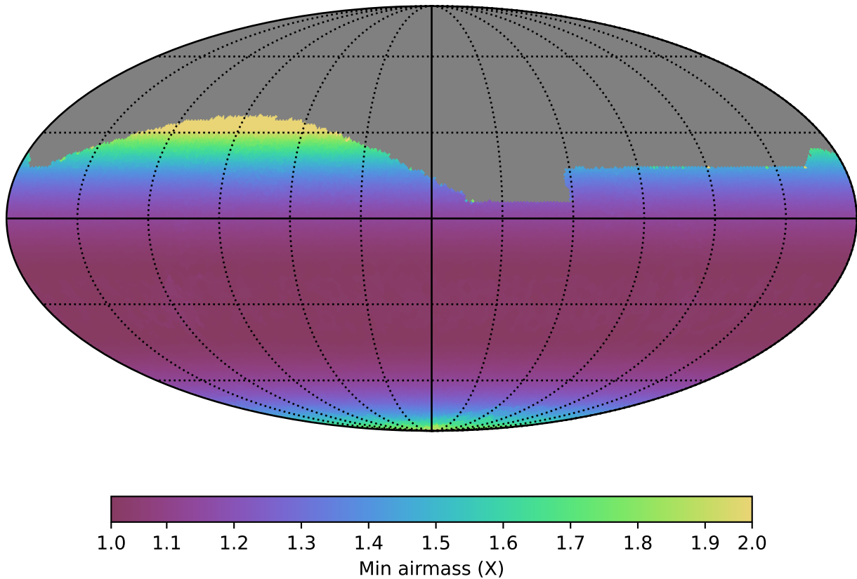
too_5_4v3.4_10yrs All sky r band: Min airmass
