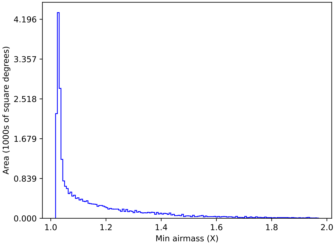
too_5_4v3.4_10yrs All sky r band: Min airmass
