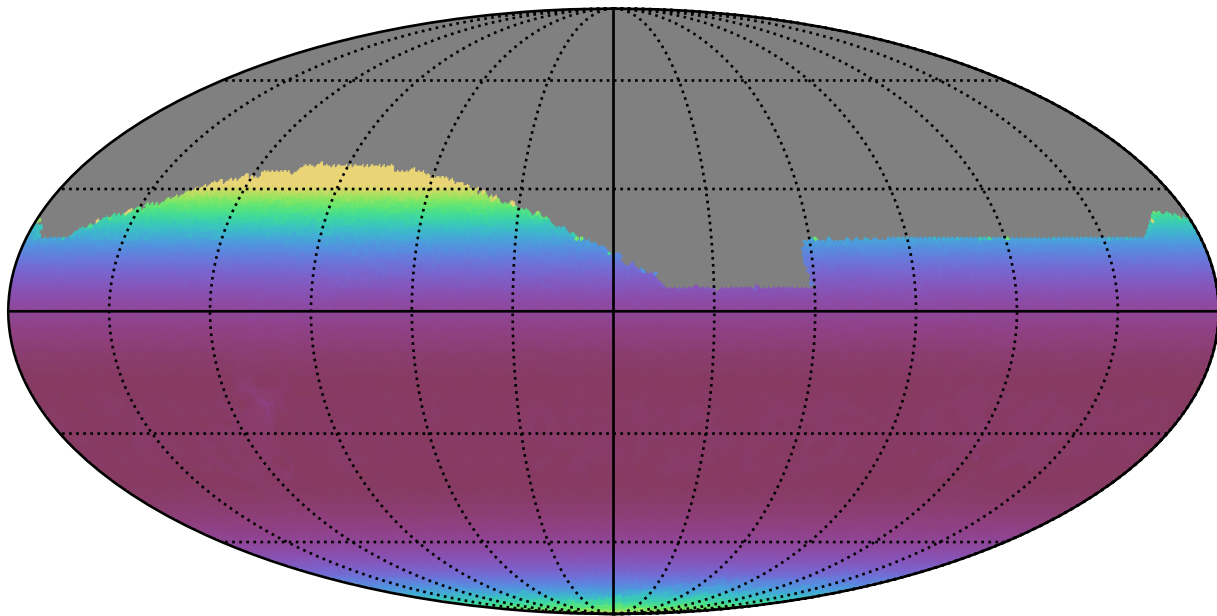
too_5_4v3.4_10yrs All sky i band: Min airmass
