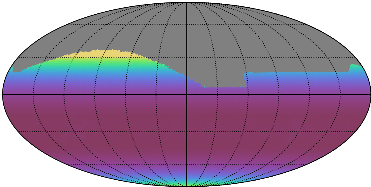
too_5_4v3.4_10yrs All sky all bands: Min airmass
