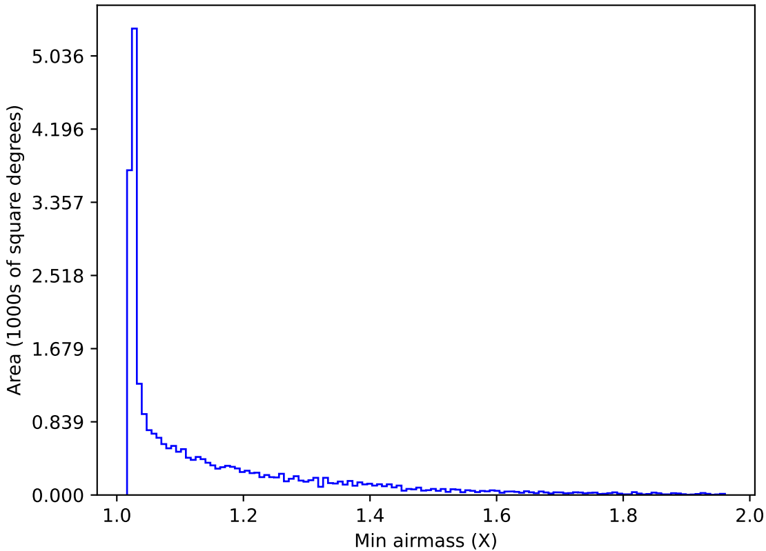
too_5_4v3.4_10yrs All sky all bands: Min airmass
