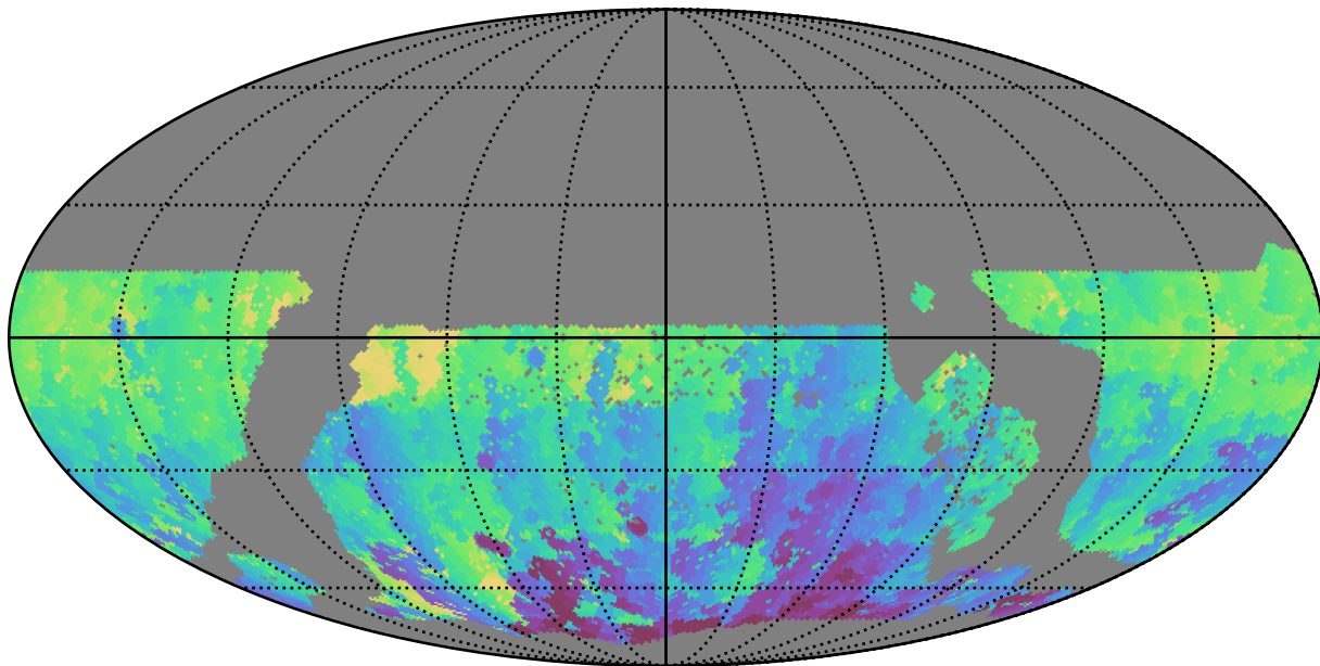
too_5_4v3.4_10yrs WFD u band: Min HA
