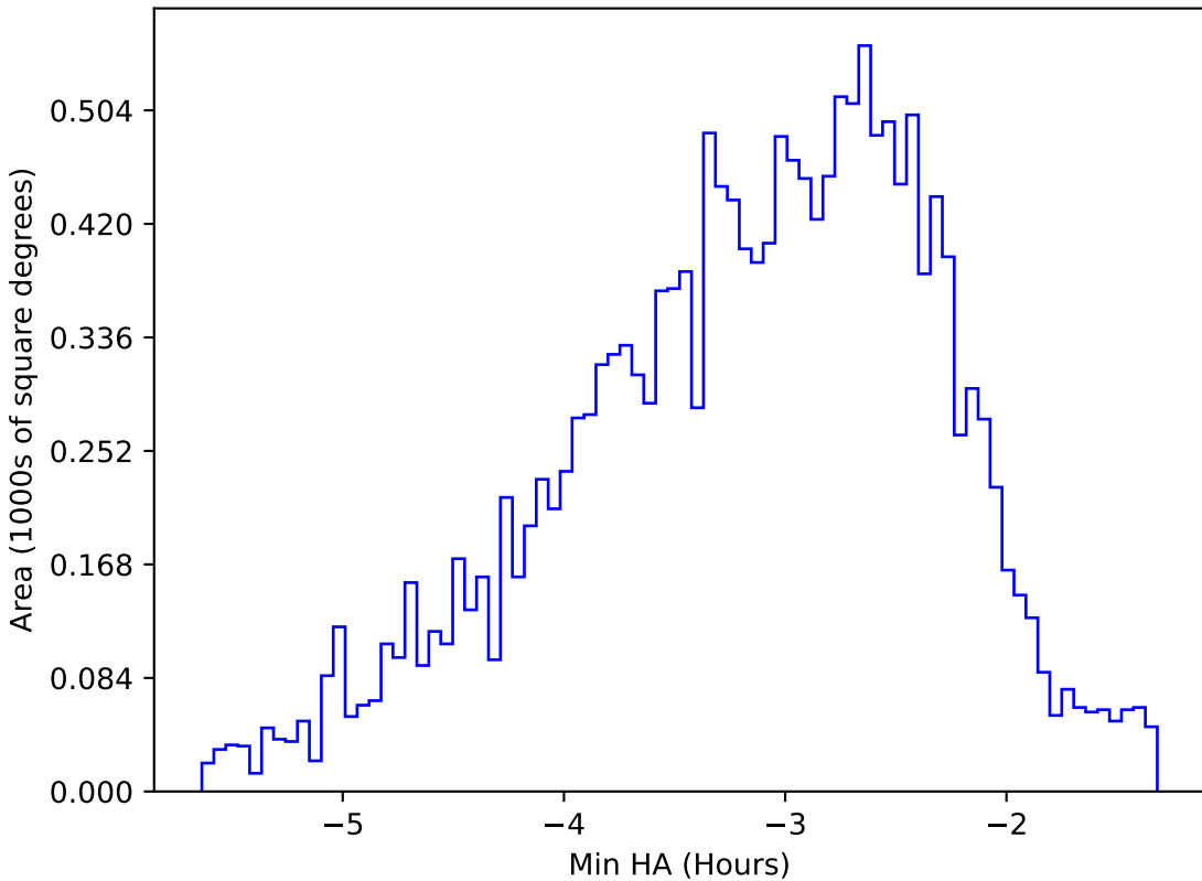
too_5_4v3.4_10yrs WFD u band: Min HA
