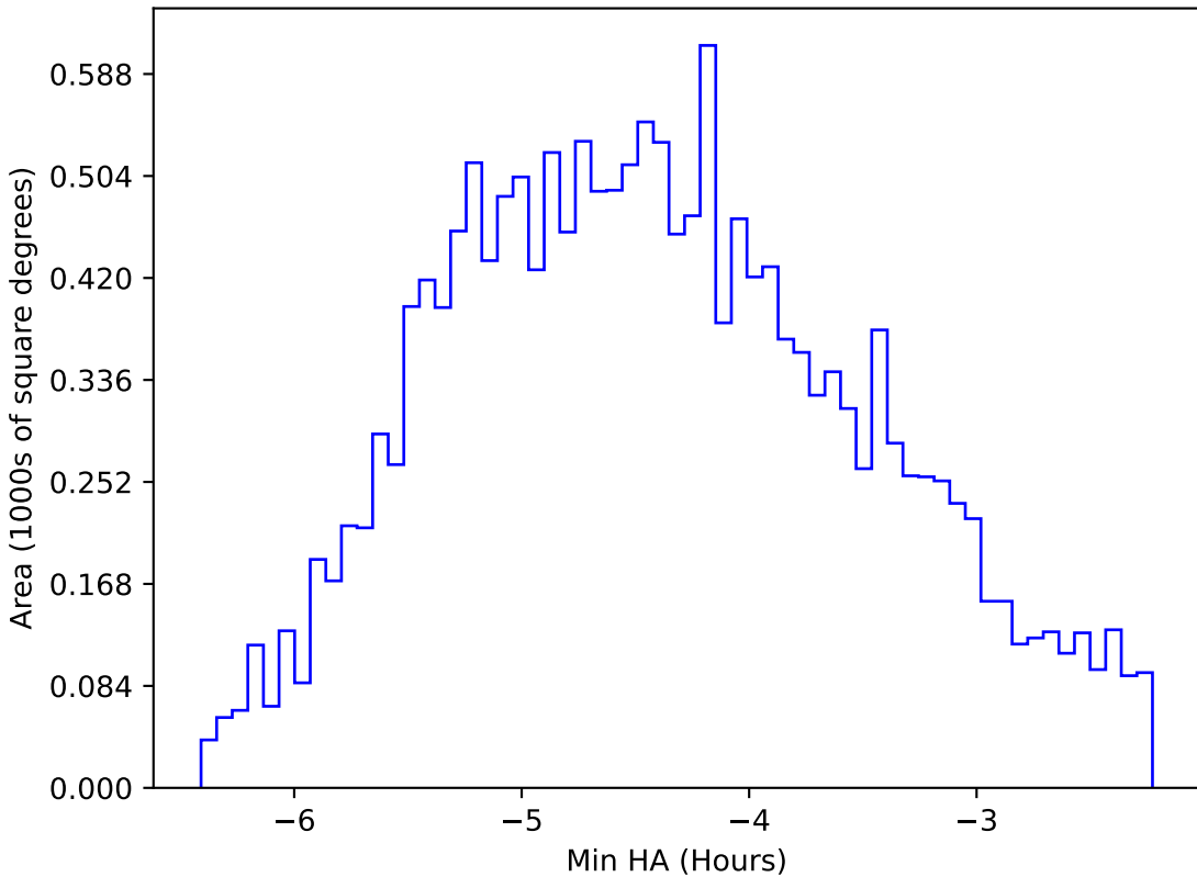
too_5_4v3.4_10yrs WFD r band: Min HA
