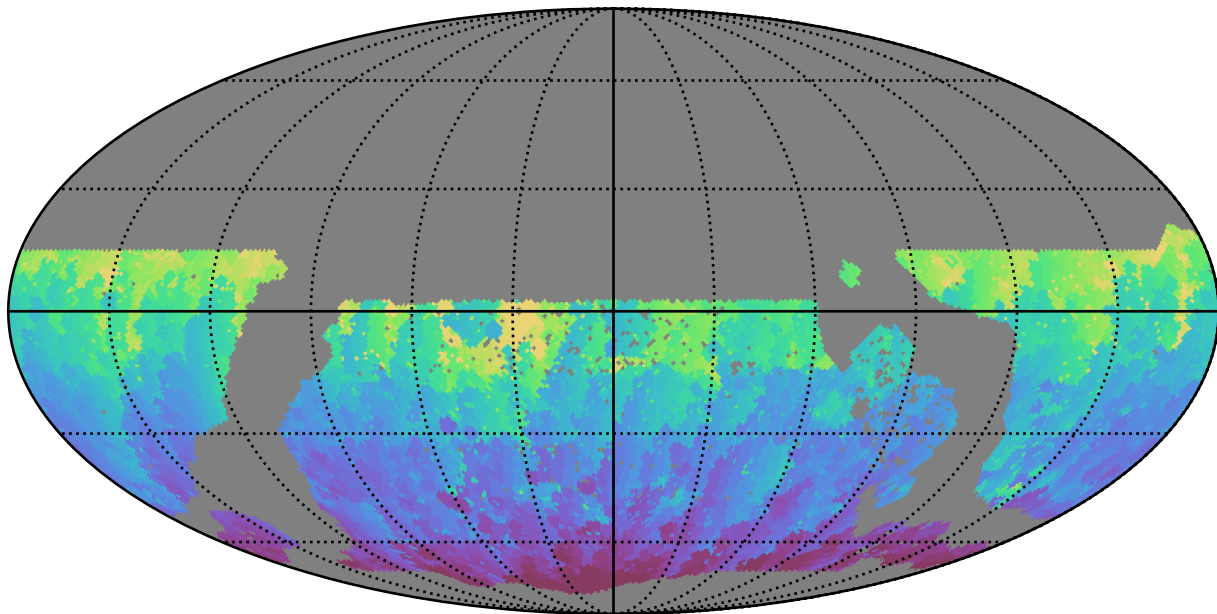
too_5_4v3.4_10yrs WFD g band: Min HA
