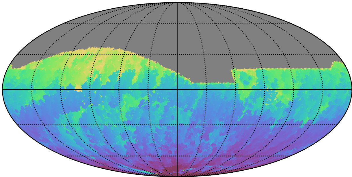
too_5_4v3.4_10yrs All sky z band: Min HA
