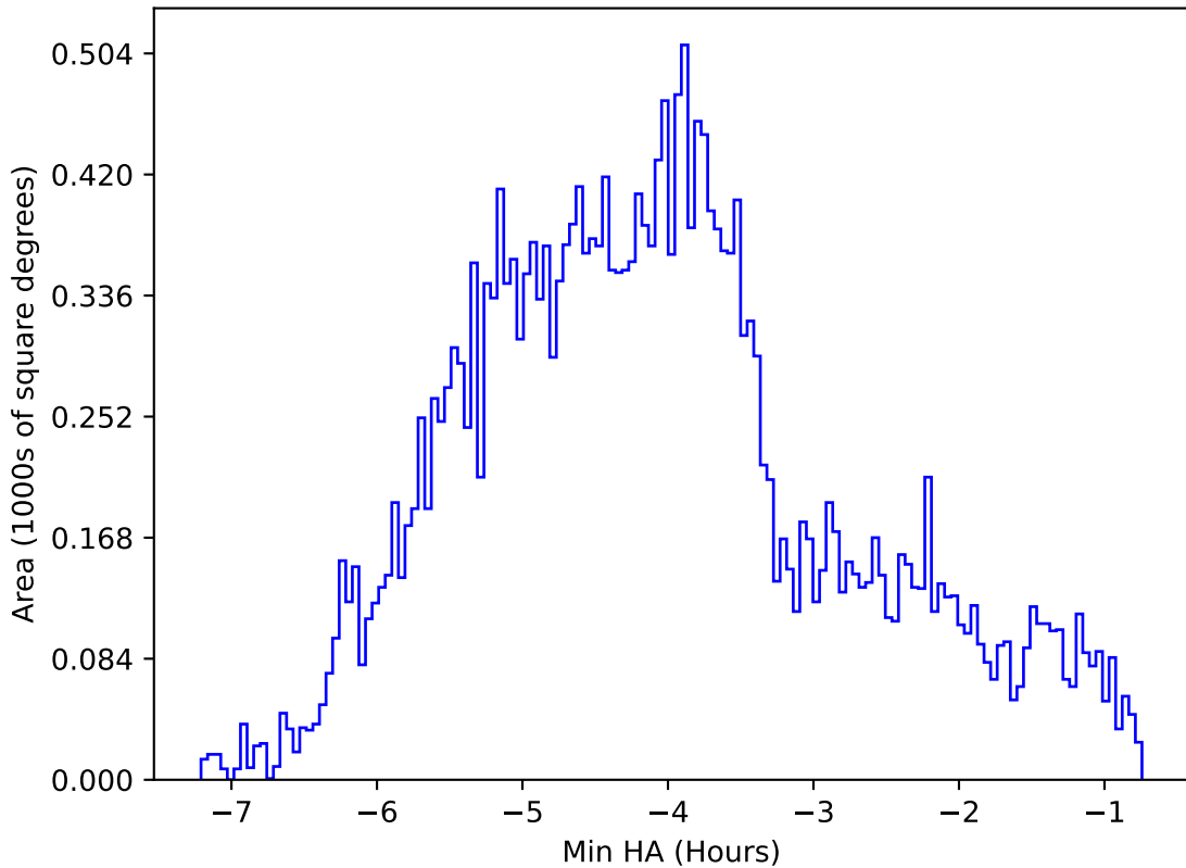
too_5_4v3.4_10yrs All sky z band: Min HA
