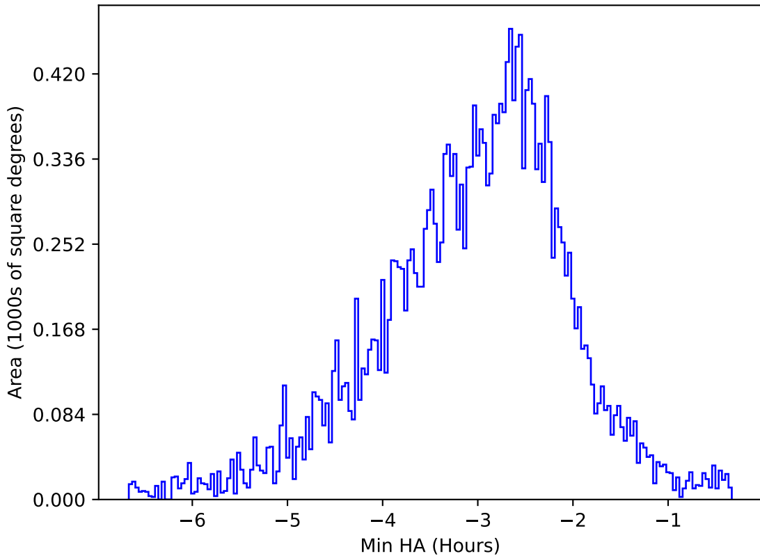
too_5_4v3.4_10yrs All sky u band: Min HA
