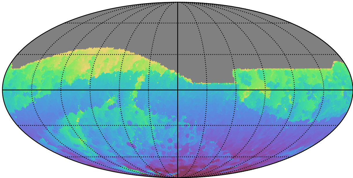
too_5_4v3.4_10yrs All sky r band: Min HA
