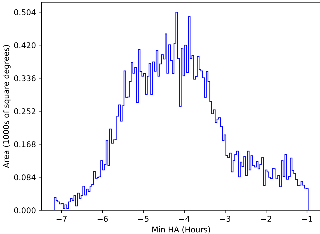
too_5_4v3.4_10yrs All sky r band: Min HA
