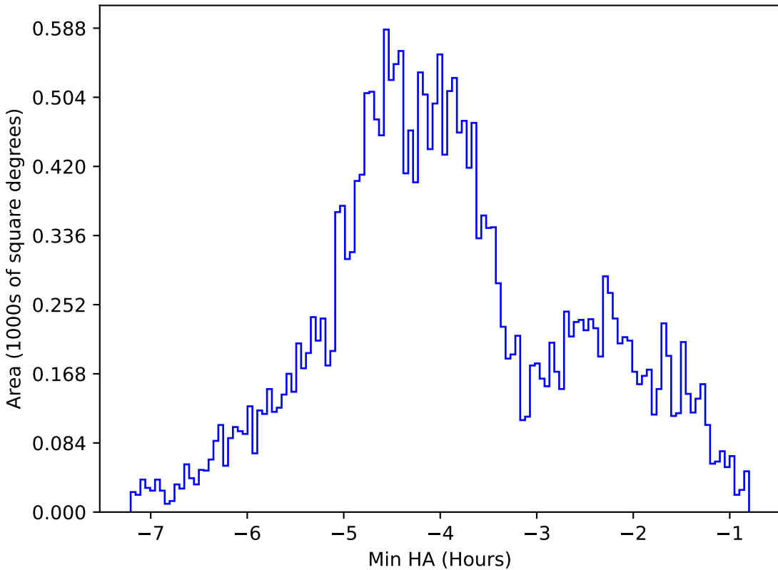
too_5_4v3.4_10yrs All sky g band: Min HA
