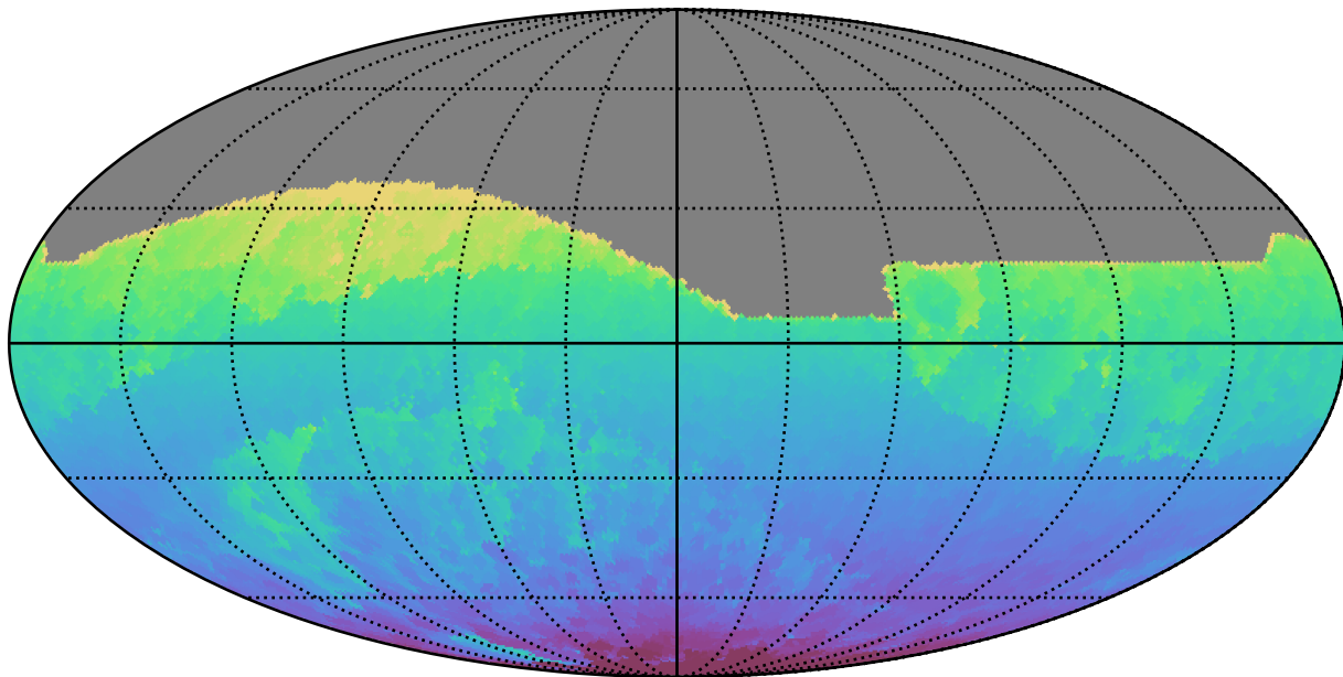
too_5_4v3.4_10yrs All sky all bands: Min HA
