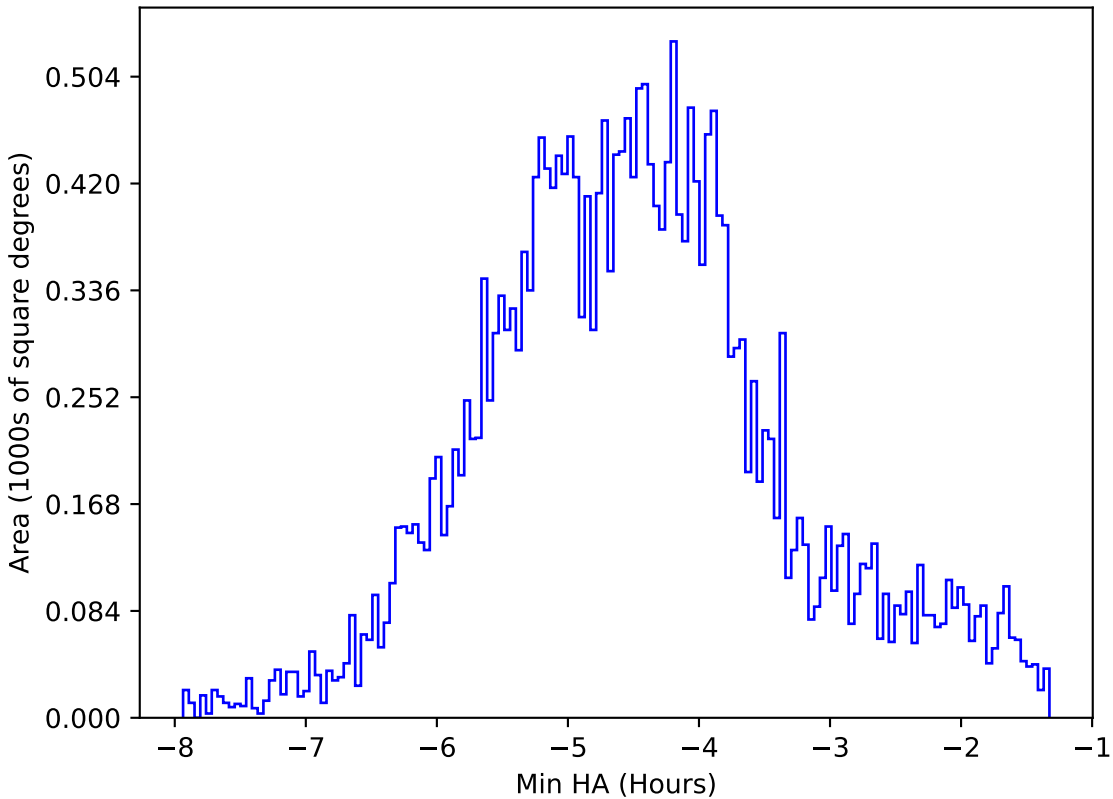
too_5_4v3.4_10yrs All sky all bands: Min HA
