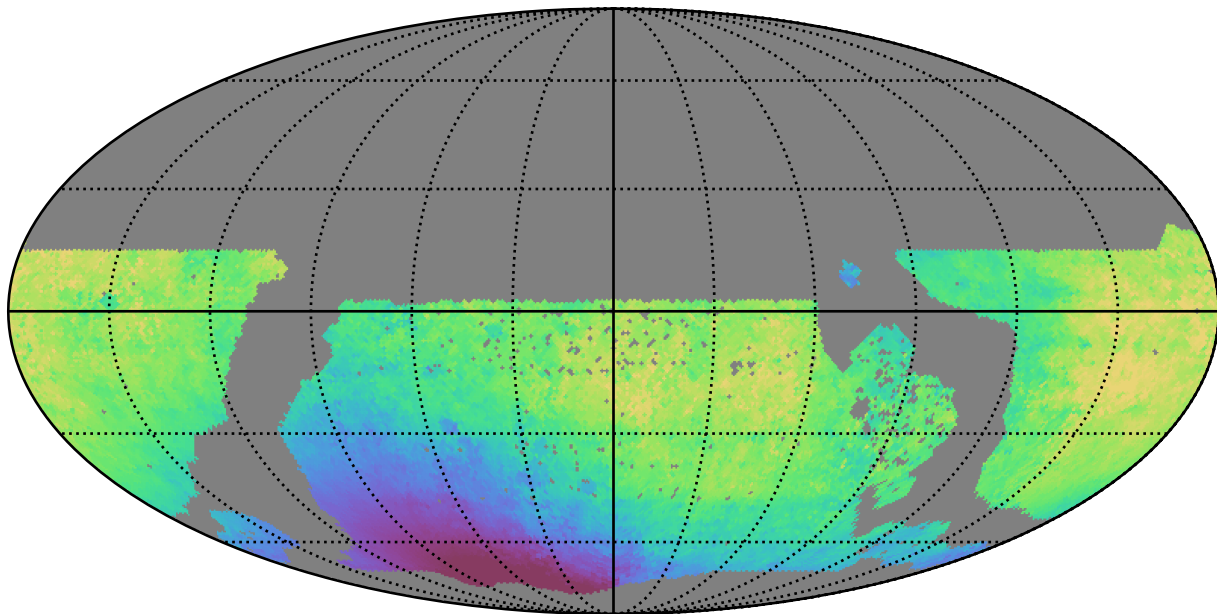
too_5_4v3.4_10yrs WFD y band: Median solarElong
