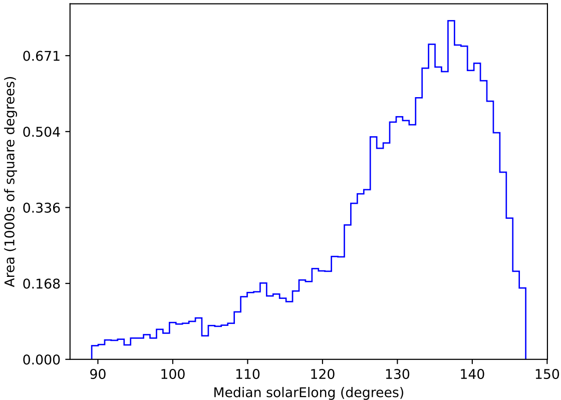
too_5_4v3.4_10yrs WFD y band: Median solarElong
