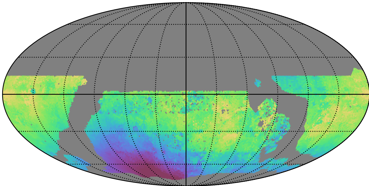
too_5_4v3.4_10yrs WFD u band: Median solarElong
