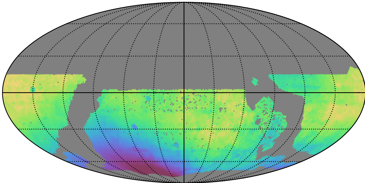
too_5_4v3.4_10yrs WFD r band: Median solarElong
