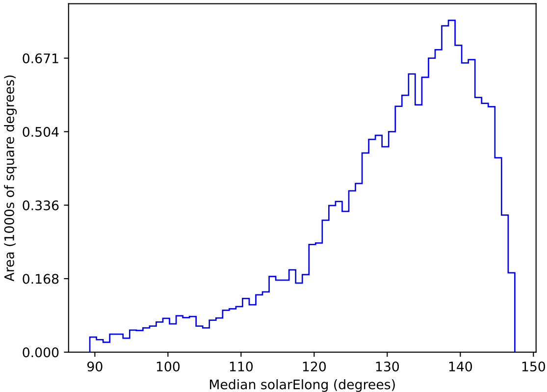
too_5_4v3.4_10yrs WFD r band: Median solarElong
