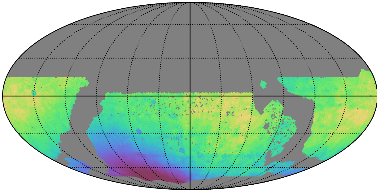
too_5_4v3.4_10yrs WFD i band: Median solarElong
