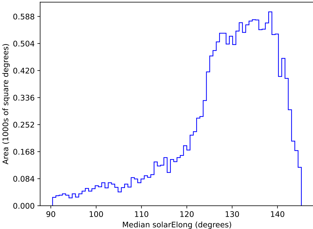
too_5_4v3.4_10yrs WFD i band: Median solarElong
