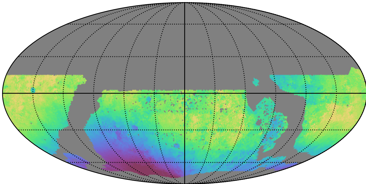
too_5_4v3.4_10yrs WFD g band: Median solarElong
