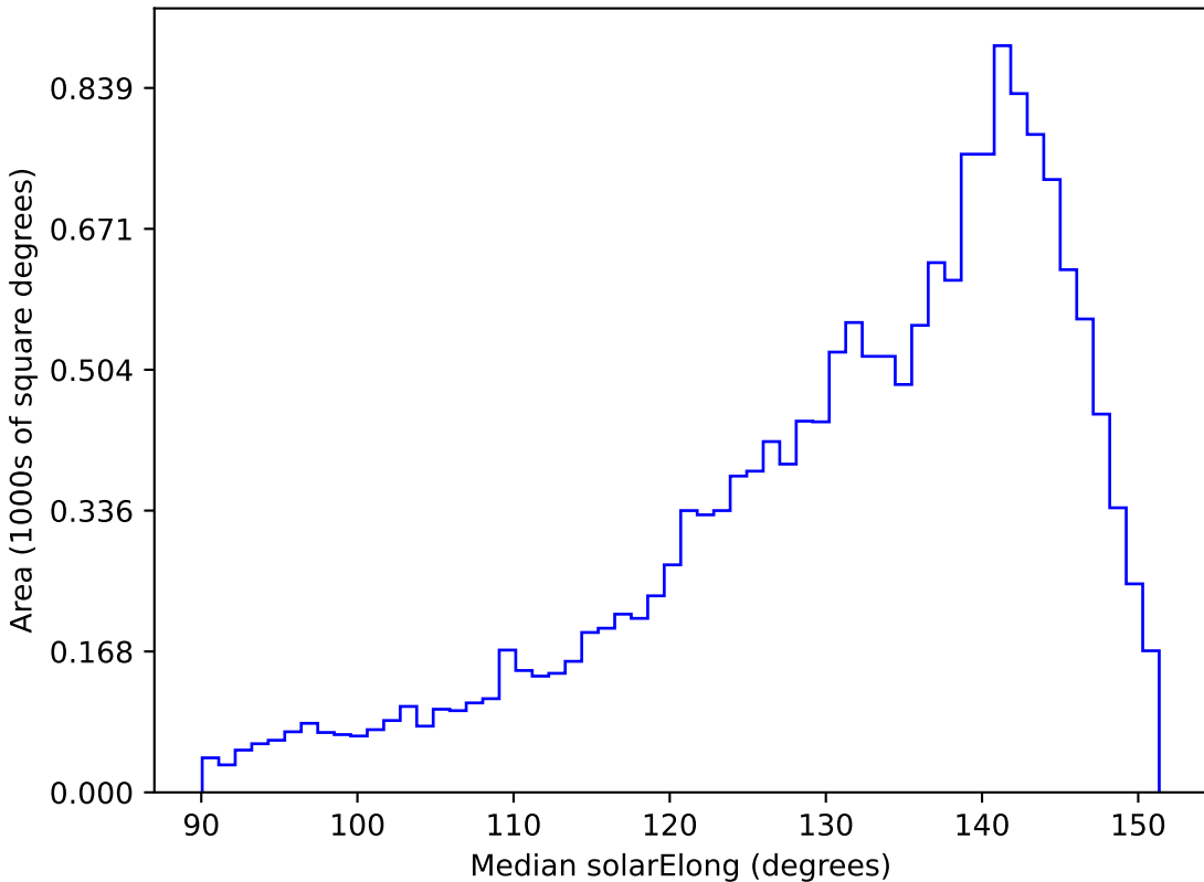
too_5_4v3.4_10yrs WFD g band: Median solarElong
