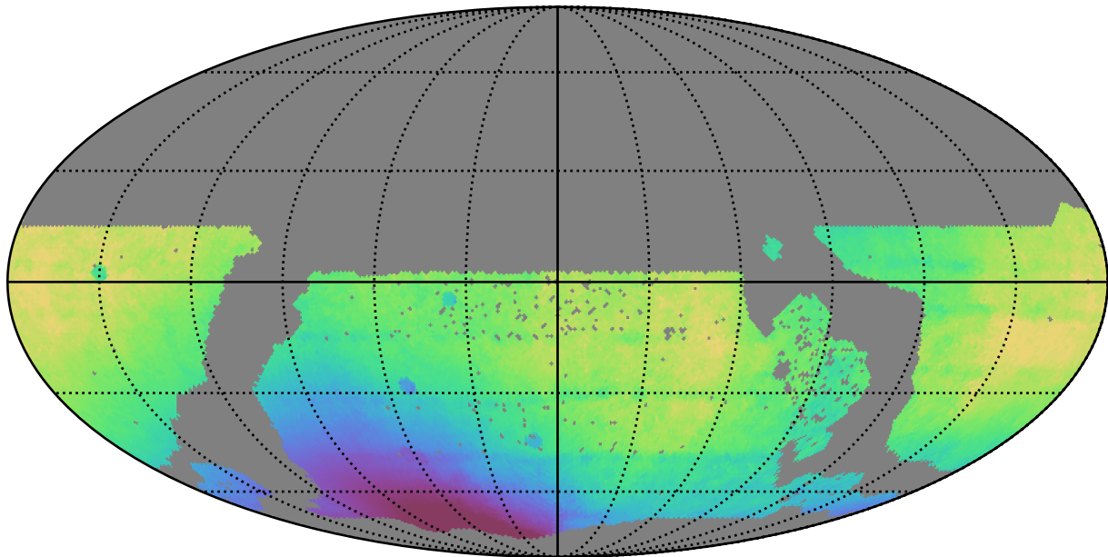
too_5_4v3.4_10yrs WFD all bands: Median solarElong
