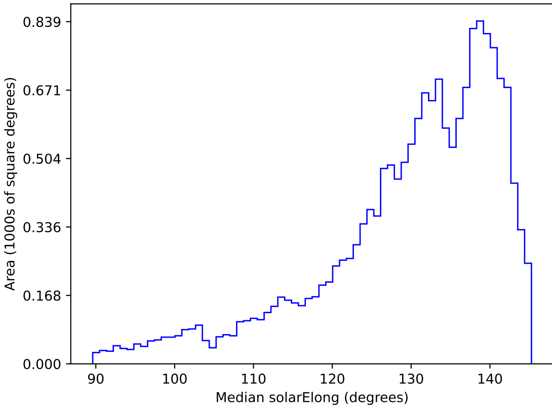
too_5_4v3.4_10yrs WFD all bands: Median solarElong
