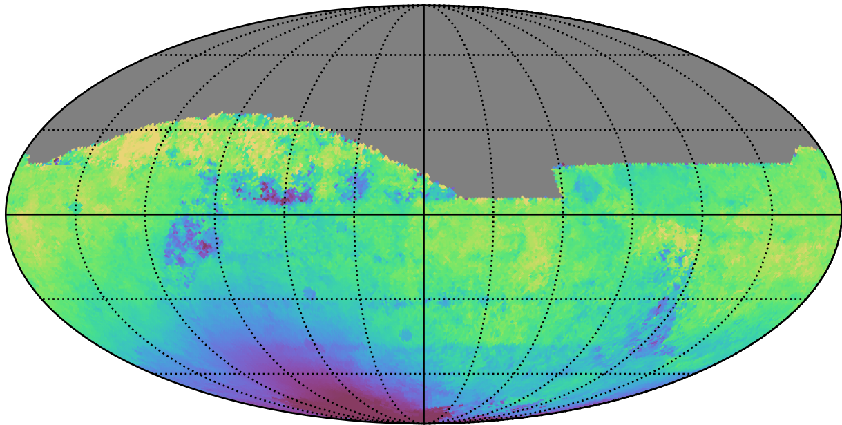
too_5_4v3.4_10yrs All sky z band: Median solarElong
