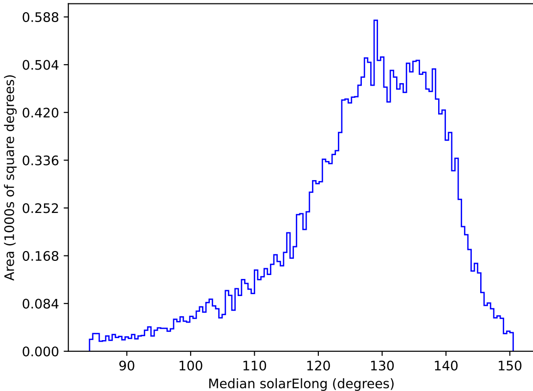
too_5_4v3.4_10yrs All sky z band: Median solarElong
