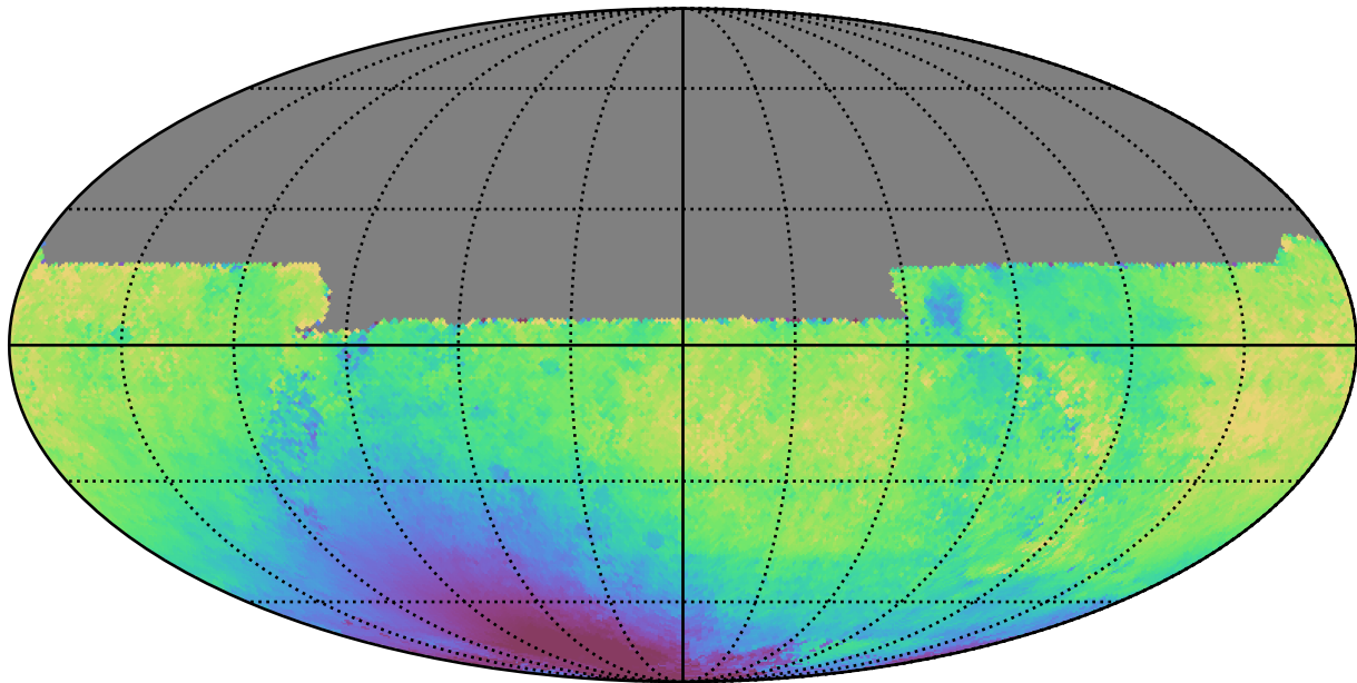
too_5_4v3.4_10yrs All sky y band: Median solarElong
